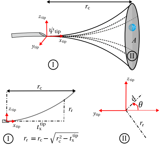
Fig. 3. Methods used for 3D needle steering. In the top figure, \psi_{tip} represents the frame attached at the tip while blue sphere represents the target. Further, r_c is defined as the radius of curvature of the circular path [5]. In inset (I), t_x^{tip} represents the distance between the plane of the control circle (plane A) and the origin of \psi_{tip} . On the other hand, r_t represents the radius of plane A. In inset (II), d and \theta represents the distance of target from the center of plane A and the angle of needle rotation, respectively. In both insets (I) and (II), blue circle represents the target. In inset (II), the gray circle at the center of the figure represents center of plane A.
