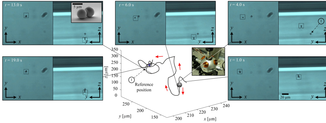
Figure 5. A representative closed-loop motion control result of a Janus micromotor (diameter of 5 \mu\text{m} ) in 3D space. Motion control is accomplished in 3D space using the electromagnetic system shown in the inset. The Janus micromotor is contained inside a capillary tube within the centre of the electromagnetic system. After t = 1 seconds, a reference position ① is given. The reference position is shown in the xy - and yz -views using a cross-hair. The black square indicates the Janus micromotor and is assigned using our feature-tracking algorithm.
