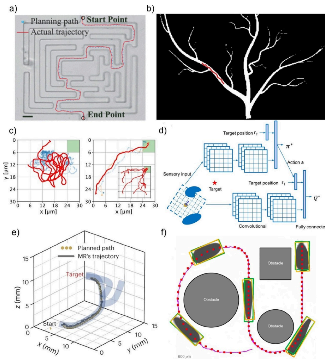
Figure 13. Autonomous micro/nanorobot navigation via machine learning. a) Path planning and navigation of a microrobot in a maze using the A* algorithm (scale bar is 20 μm). Reproduced from ref 907, Copyright 2018 IEEE. b) Simulation of path planning in a plant vein structure using RRT*-Connect. Reproduced with permission under a Creative Commons CC-BY License from ref 986, Copyright 2023 Frontiers. c) Learning process for the navigation of a self-thermophoretic microrobot using Q-learning. Reproduced from ref 972, Copyright 2021 American Association for the Advancement of Science. d) Neural network architecture of a DRL algorithm for the navigation of various micro/nanorobots. Reproduced with permission under a Creative Commons CC-BY License from ref 992, Copyright 2020 WILEY-VCH. e) Path planning and reinforcement learning for fully autonomous navigation of a magnetic microrobot. Reproduced from ref 968, Copyright 2024 Springer Nature. f) Supervised learning for autonomous navigation of a magnetic nanorobot swarm around obstacles. Reproduced from ref 995, Copyright 2022 Springer Nature.
